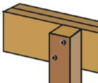
Image E: For a sturdy beam, secure posts to beams with offset carriage bolts. Notice the 12 3/4" overhang.
