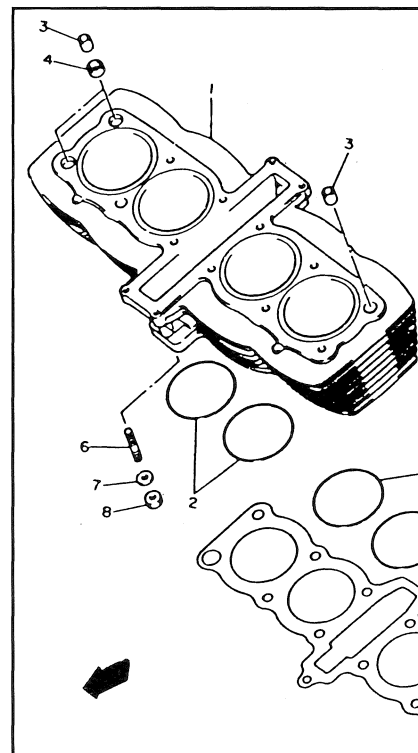
BLOC-CYLINDRES
